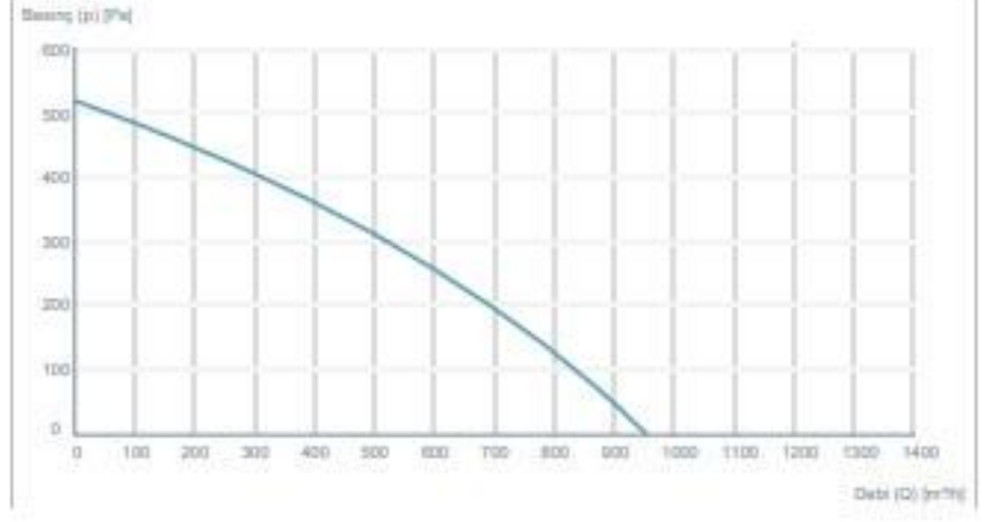
REC 40-20 A
