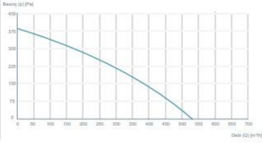
REC 30-15
