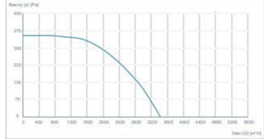
REC 60-35
